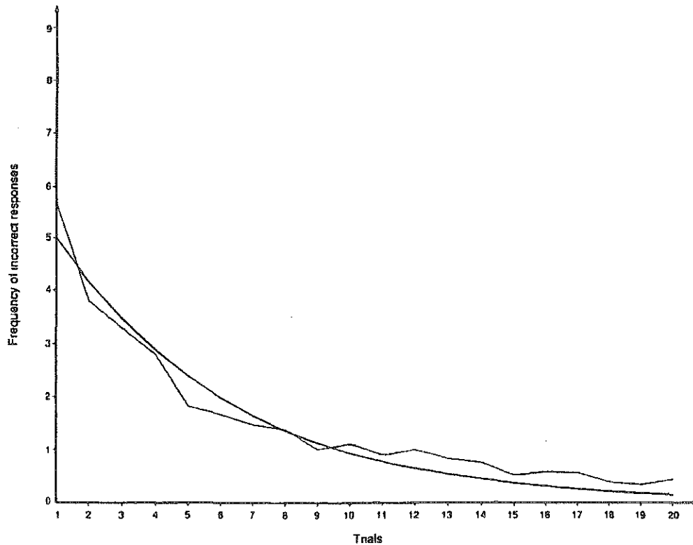
FIG. 1.3. Multiplication exercises at grade level 3.95, sample size = 406, \hat{q} = .500 , \hat{\alpha} = 0.831 .
