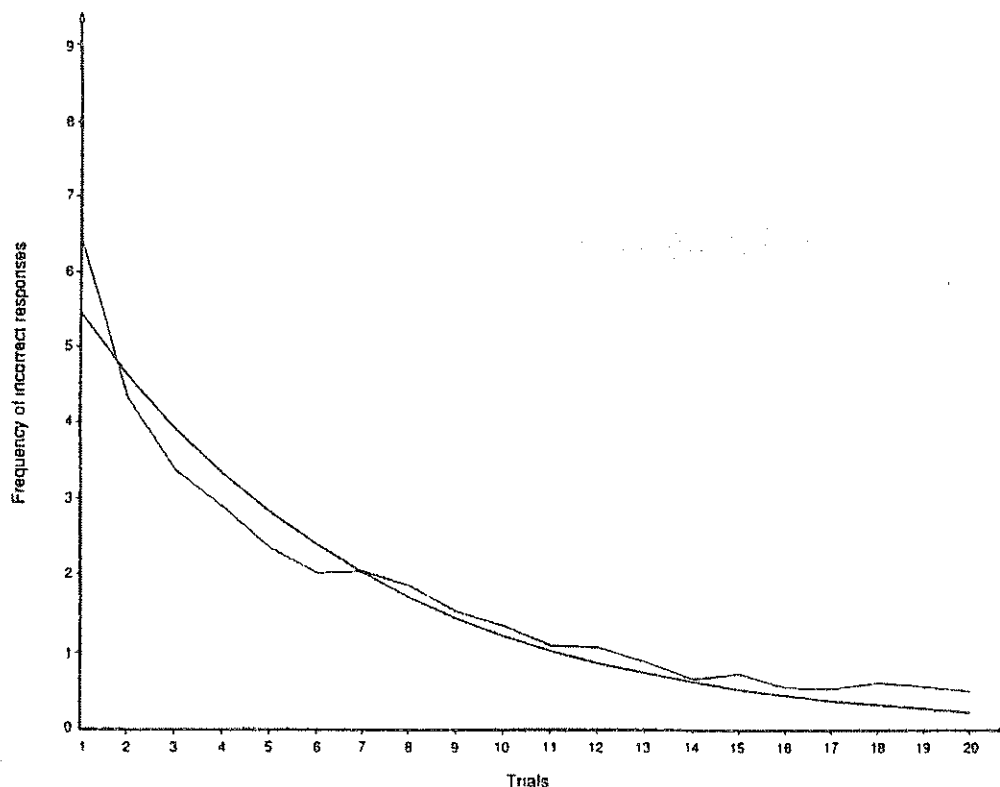
FIG. 1.1. Addition at grade-level 3.65, sample size = 612, \hat{q} = 0.545 , \hat{\alpha} = 0.847 .
